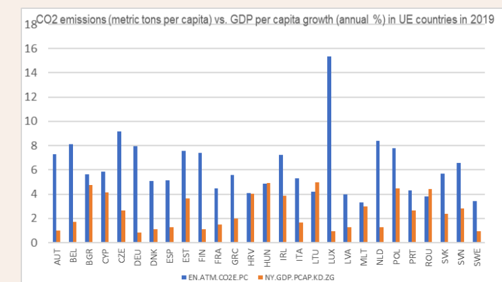
Fig. 3. A comparative analysis of CO 2 emissions (metric tons per capita) vs. GDP per capita growth (annual %) in EU countries in 2019
