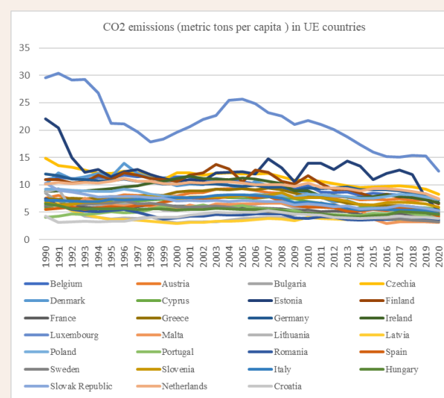
Fig. 2. CO 2 emissions (metric tons per capita) in European countries in the period 1990-2020
