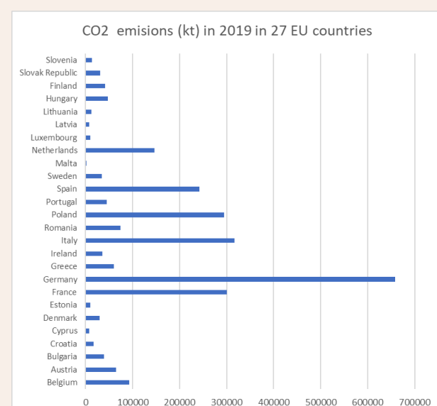
Fig. 1. CO 2 emissions (kt) in European countries in 2019
